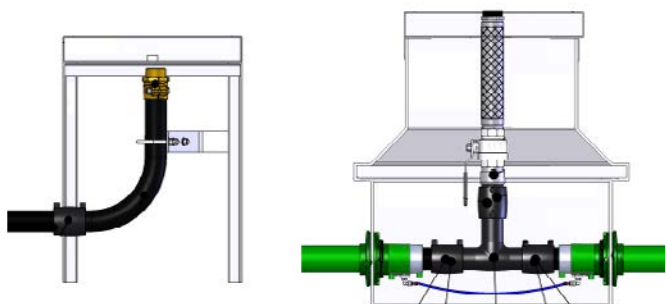
A plastic bend in a suction system and a flexible connector in a pressure system.
