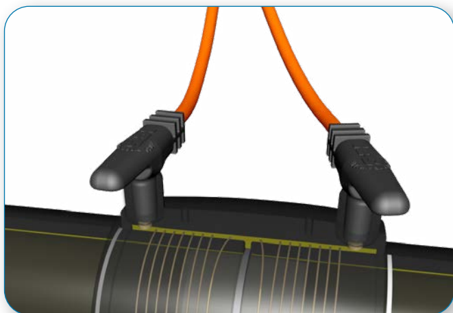
During electrofusion welding material is melted by the heat from the socket wiring and the pipe fuses with the welding socket.
