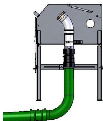
Example of a good filling point installation.
