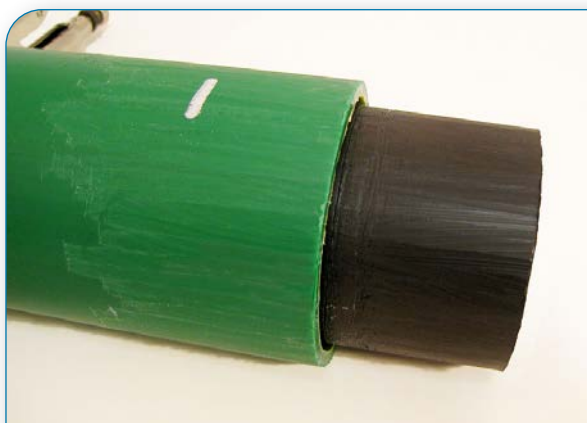
Correctly scraped pipes. Oxide has been removed from the whole area to be welded.
