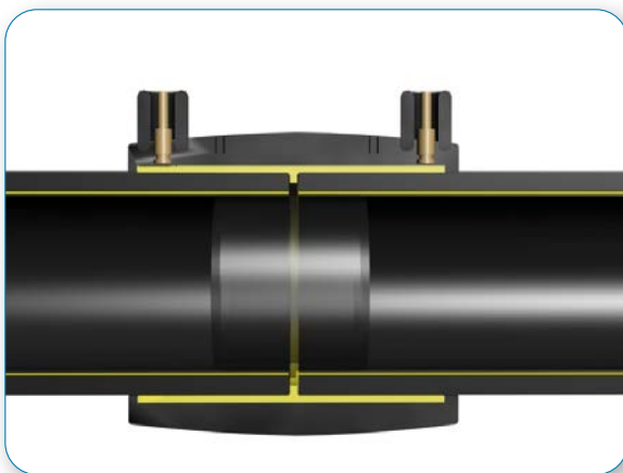
Conductive connectors should be inserted in every joint.
