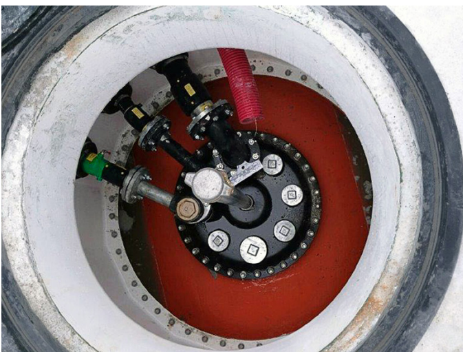
Control and monitoring of the interstitial space between the inner and outer pipes, provided an extra layer of security
